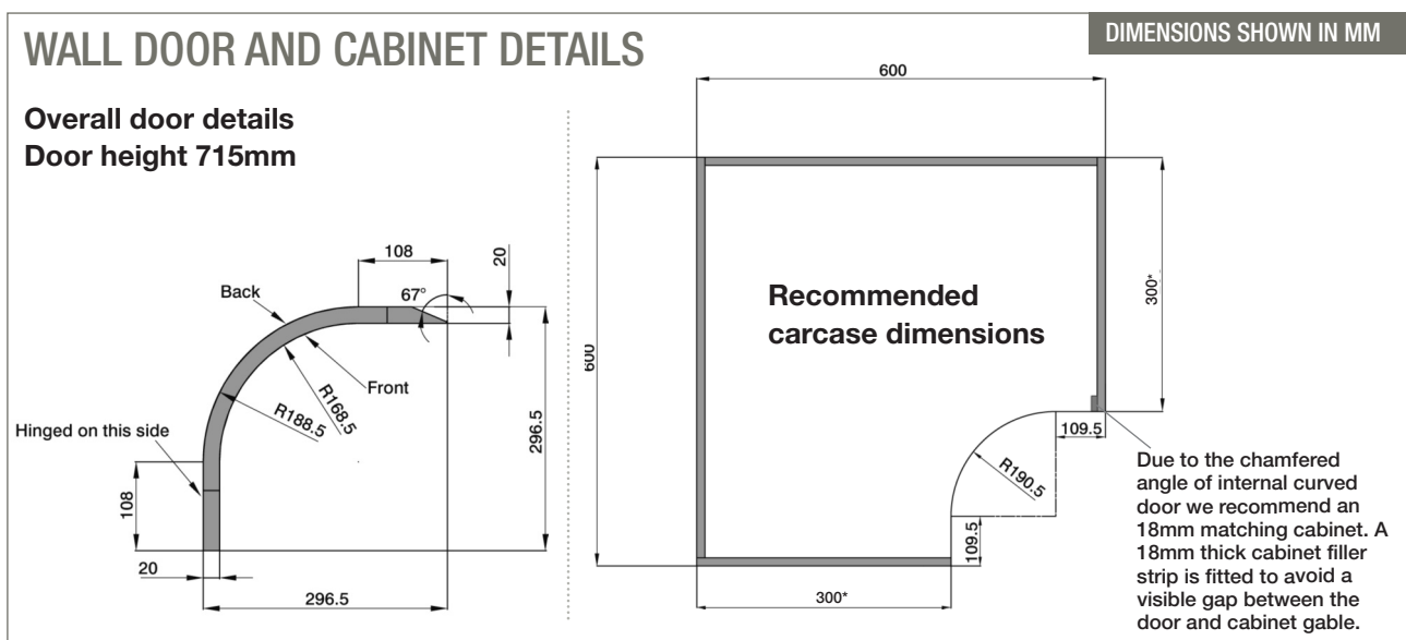
A carcass jig is available - ICJIG600
